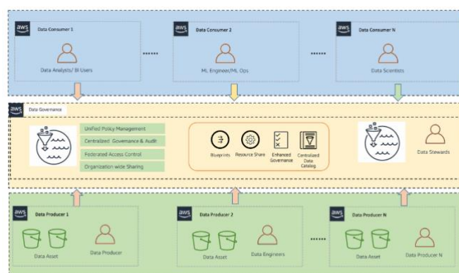
A high-level design of data mesh in AWS.
