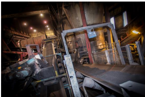
Left, the Belt Conveyor System (BCS) installed in an underground mine. Right, Time of Flight camera that captures 3D point cloud data.
